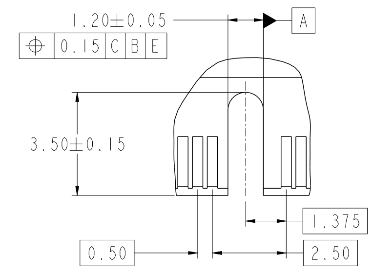
DETAIL E SCALE 12:1
