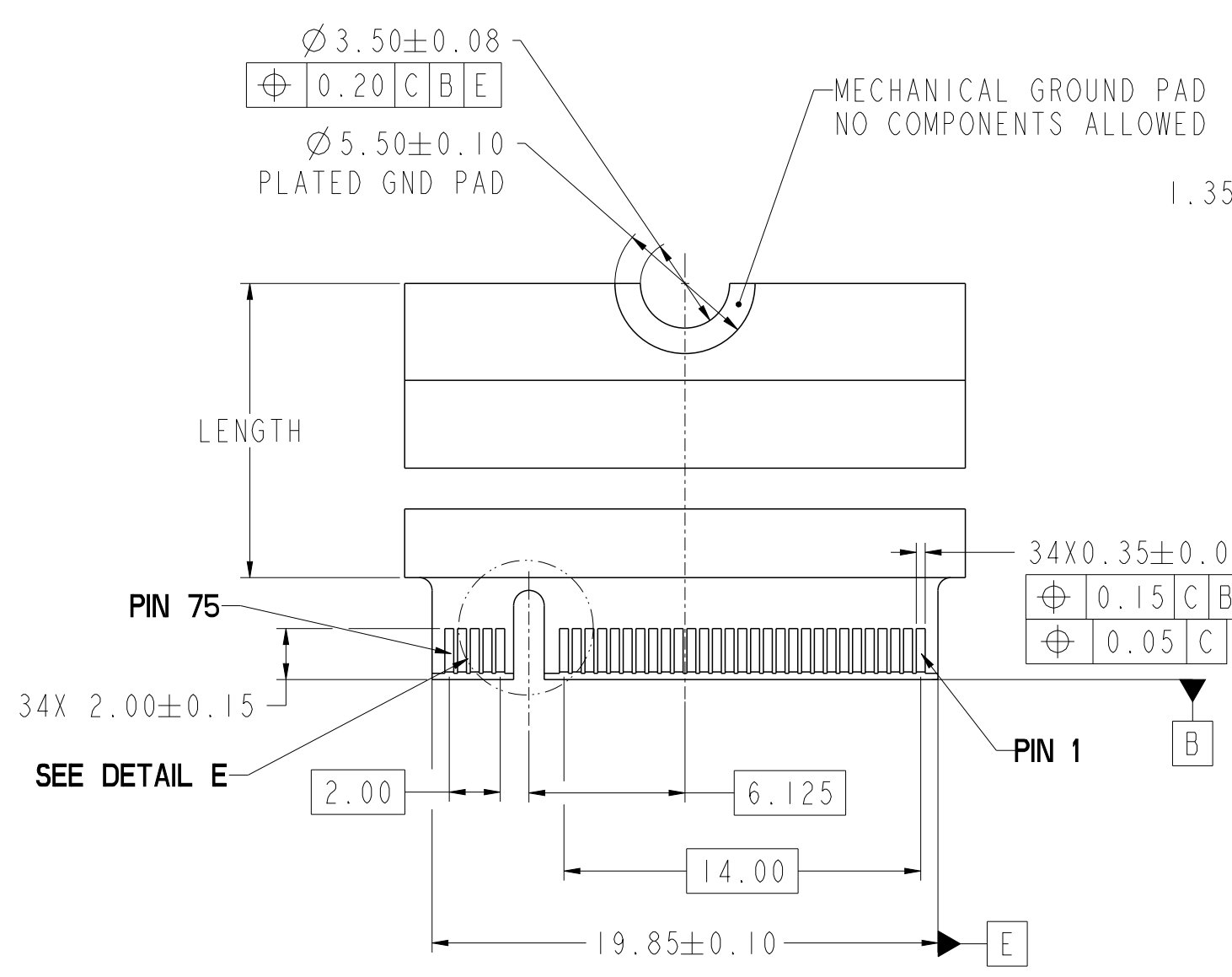
TOP VIEW OF CARD
