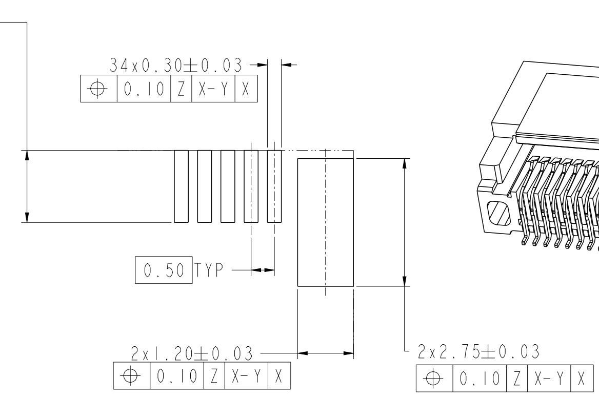
DETAIL D SCALE 12:1
