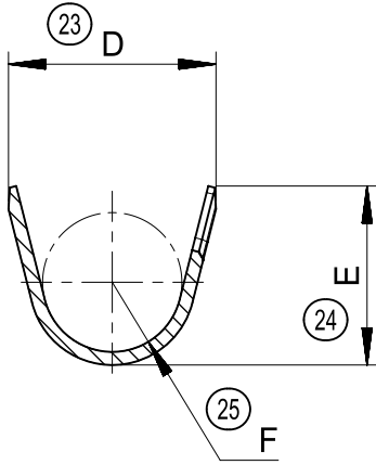
SECTION B-B
