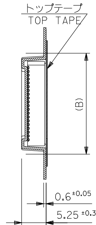
SECT. Z-Z
