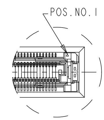
DETAIL C (SCALE 2:1)
