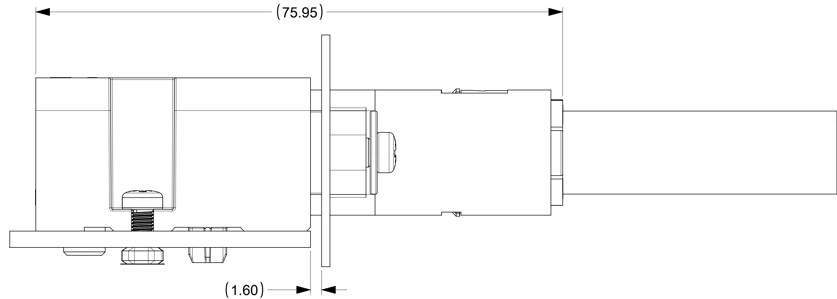
ASSEMBLED AND MATED WITH RA HEADER_SOLDER TAIL VERSION (2155106241)
