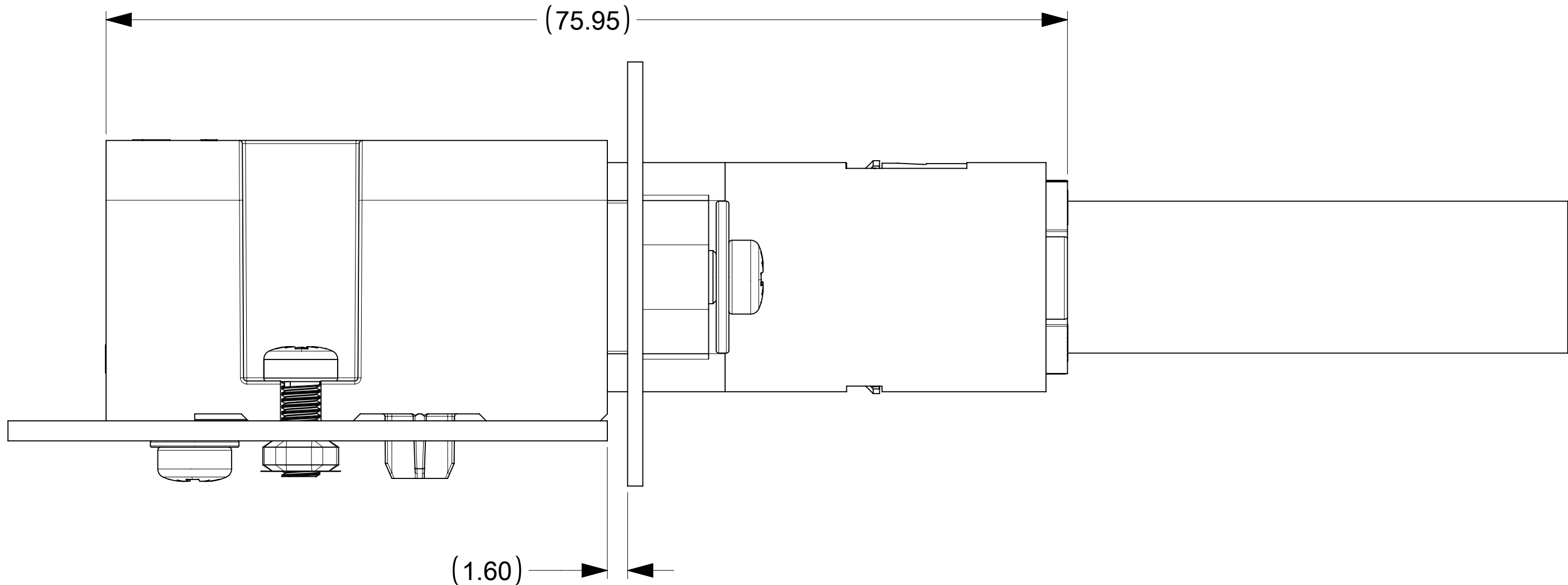
ASSEMBLED AND MATED WITH RA HEADER_SCREW MOUNT VERSION (2155106031)
