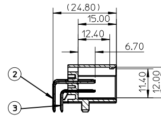
SECTION Z-Z
