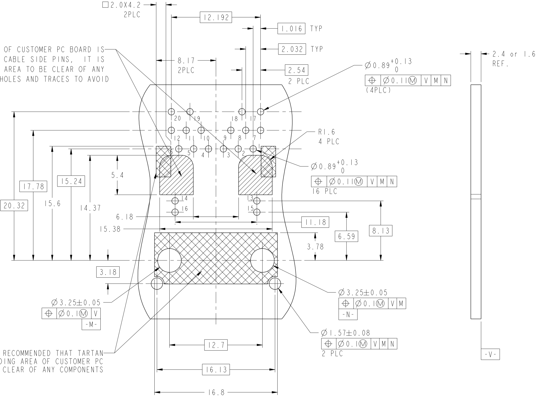
SUGGESTED PCB FOOTPRINT COMPONENT SIDE
