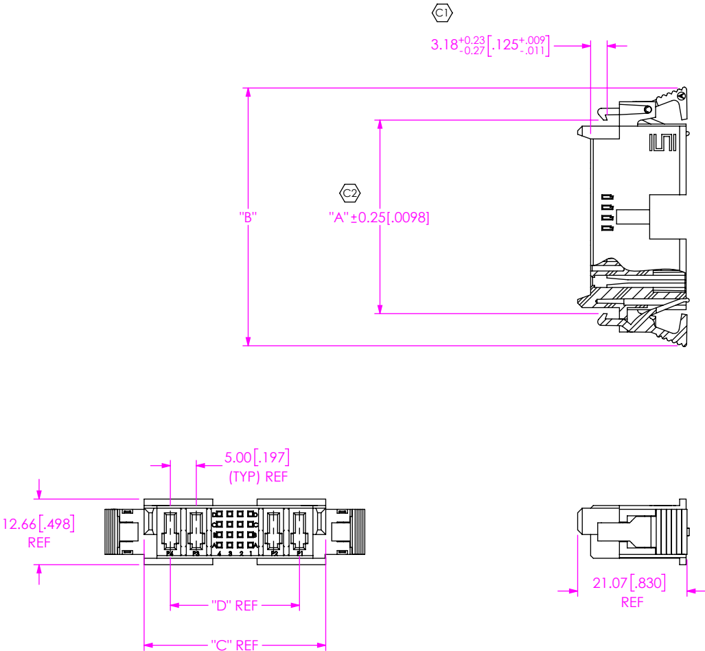
FIG 1 IMSC5-02-16-02-L SHOWN
