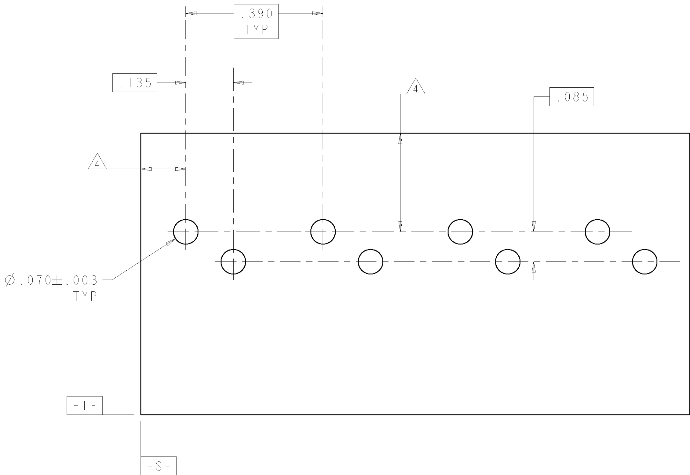
SUGGESTED PRINTED CIRCUIT BOARD MOUNTING DIMENSIONS (VIEWED FROM SOLDER SIDE)
