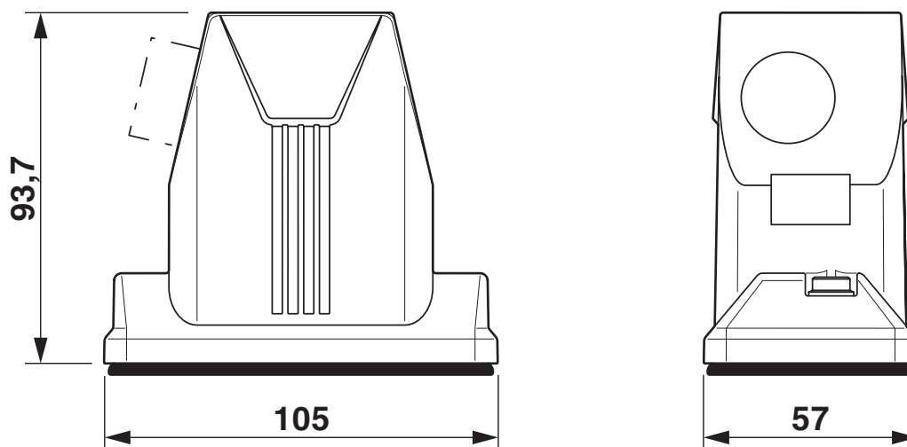
Dimensional drawing
