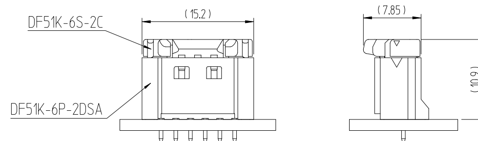
ENGAGEMENT FIGURE (2:1)
