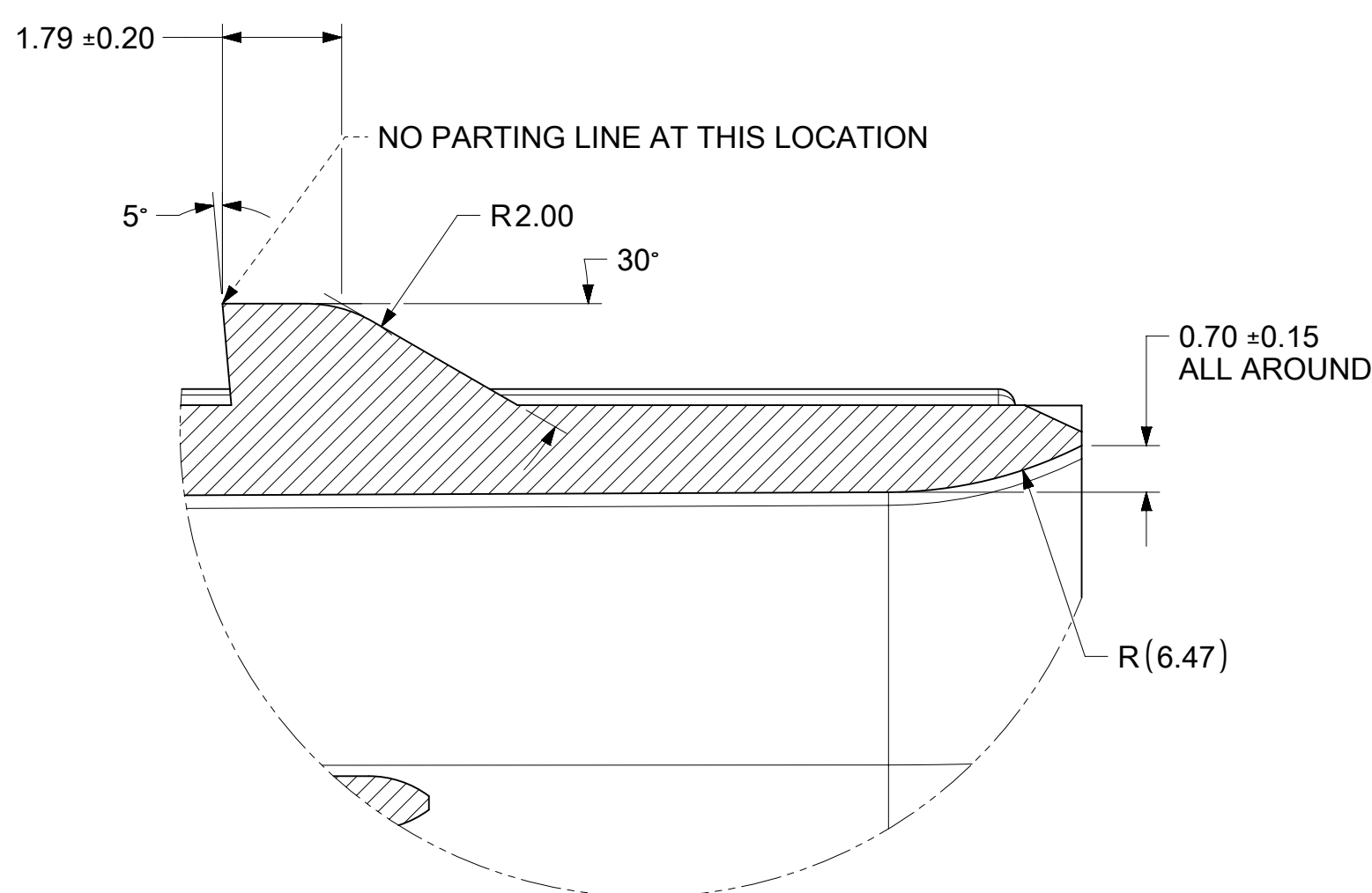
DETAIL 3 SCALE 10:1
