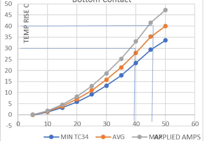
Temp Rise for applied Current TD 3 and 4 Bottom Contact
