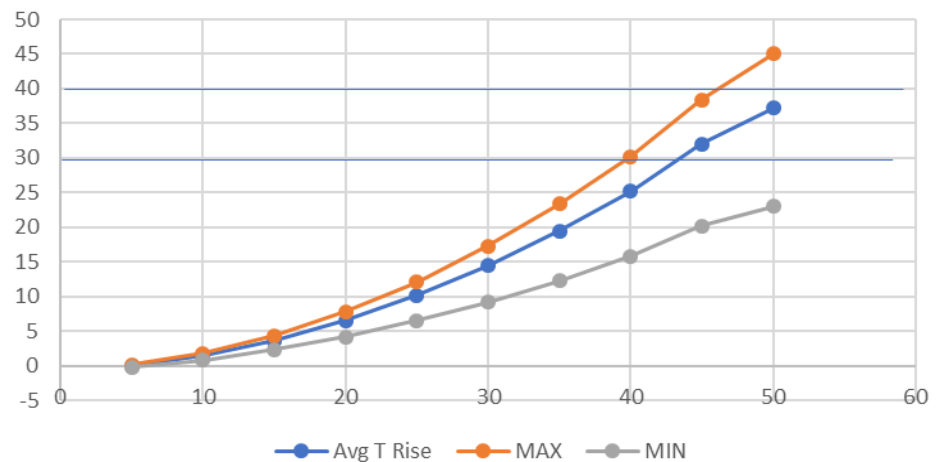
Temp Rise for Applied Current Group 4
