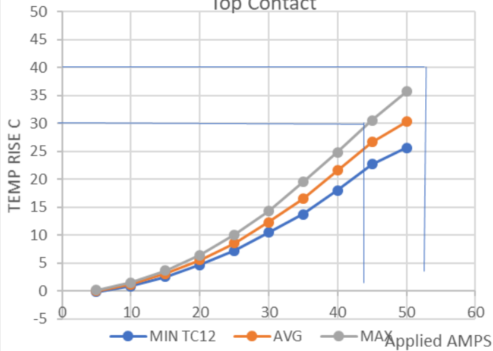
Temp Rise for applied Current TD 1 and 2 Top Contact
