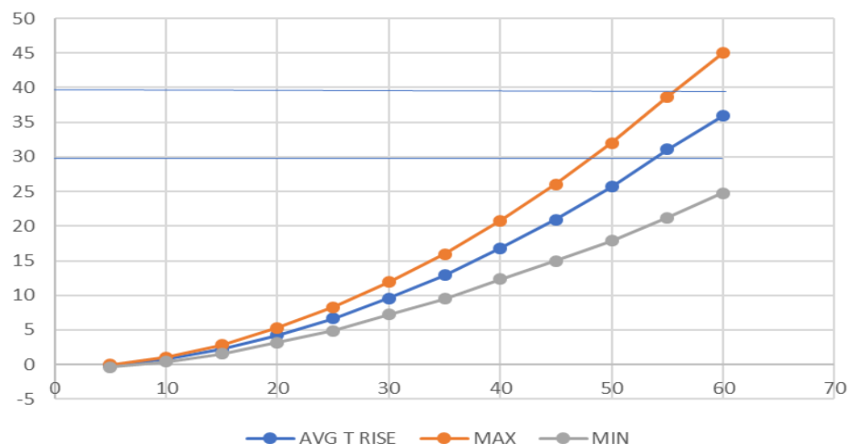
TEMP RISE FOR APPLIED CURRENT GP 8
