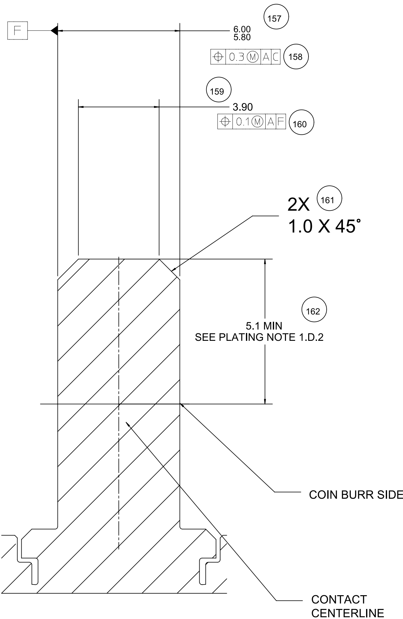
SECTION CB-CB
