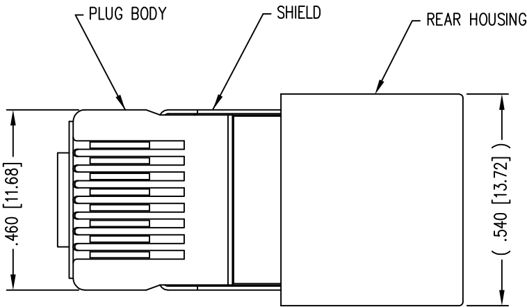
( SHOWN ASSEMBLED )
