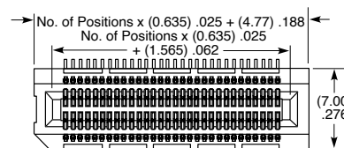
10, 20, 30 & 40 POSITIONS
