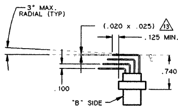
TERMINATION POSTS BENT 90° IN "B" DIRECTION FLANGED MTC50-BF/SX-PX3
