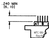
TERMINATION POSTS .240 MINIMUM LENGTH FLANGELESS MTC50-BJX-PX2
