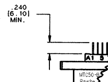
TERMINATION POSTS .240 MINIMUM LENGTH FLANGED MTC50-BF/SX-PX2
