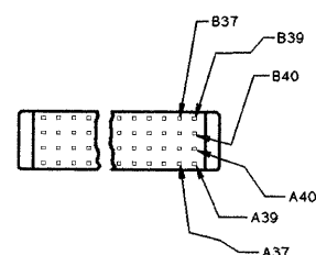
TERMINATION POSTS .240 MINIMUM LENGTH FLANGED MTC50-BF/SX-PX2
