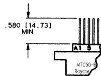
TERMINATION POSTS .580 MINIMUM LENGTH FLANGELESS MTC50-BJX-PX1
