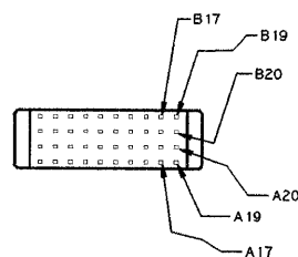
TERMINATION POSTS .580 MINIMUM LENGTH FLANGED MTC50-BF/SX-PX1
