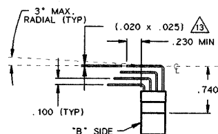
TERMINATION POSTS BENT 90° IN "B" DIRECTION FLANGELESS MTC50-BJX-PX3
