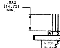
TERMINATION POSTS .580 MINIMUM LENGTH FLANGED MTC50-BF/SX-PX1
