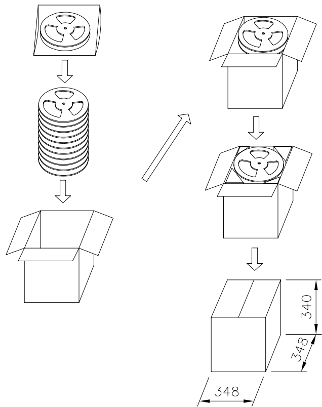
PACKAGING PROCESS
