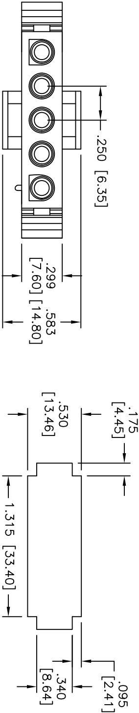
Panel hole dimensions
