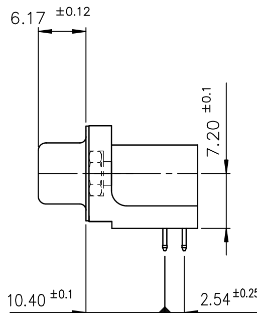
PC card drilling dimensions(after plating)
