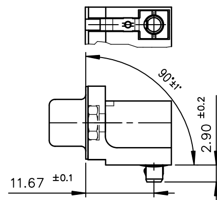
Detail of grounding strip
