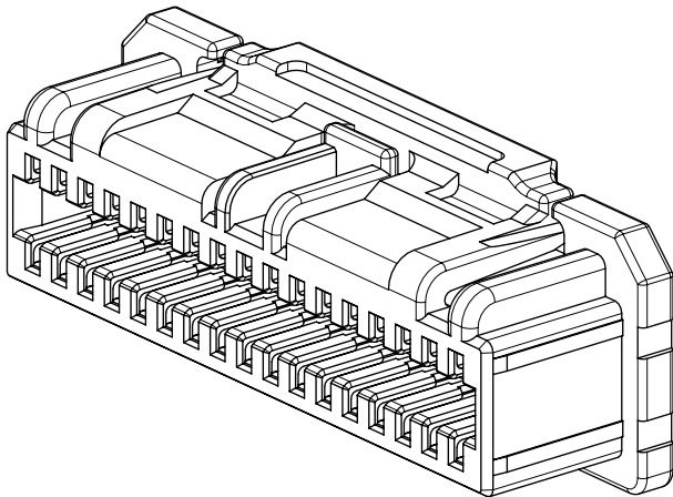
34-40極 34-40 CIRCUIT
