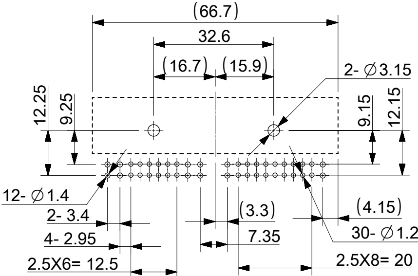
PCB LAYOUT General Tolerance: ±0.05
