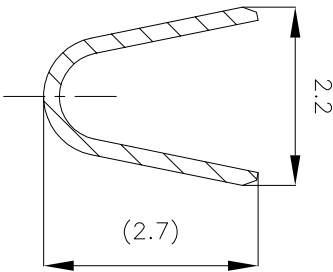
SECT "B"-"B"
