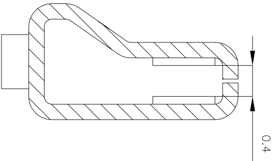
SECT "C"-"C"
