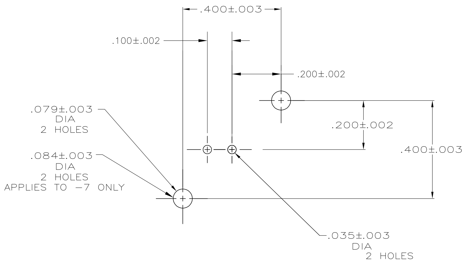
PCB CONFIGURATION
