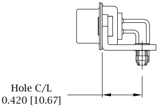
Boardlock Brackets Come Assembled On Connector
