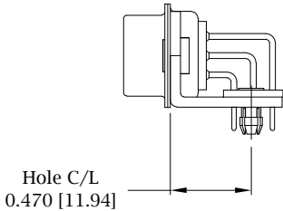
50 Position Connector Boardlock Bracket ** 50 Position Comes With Locator Plate
