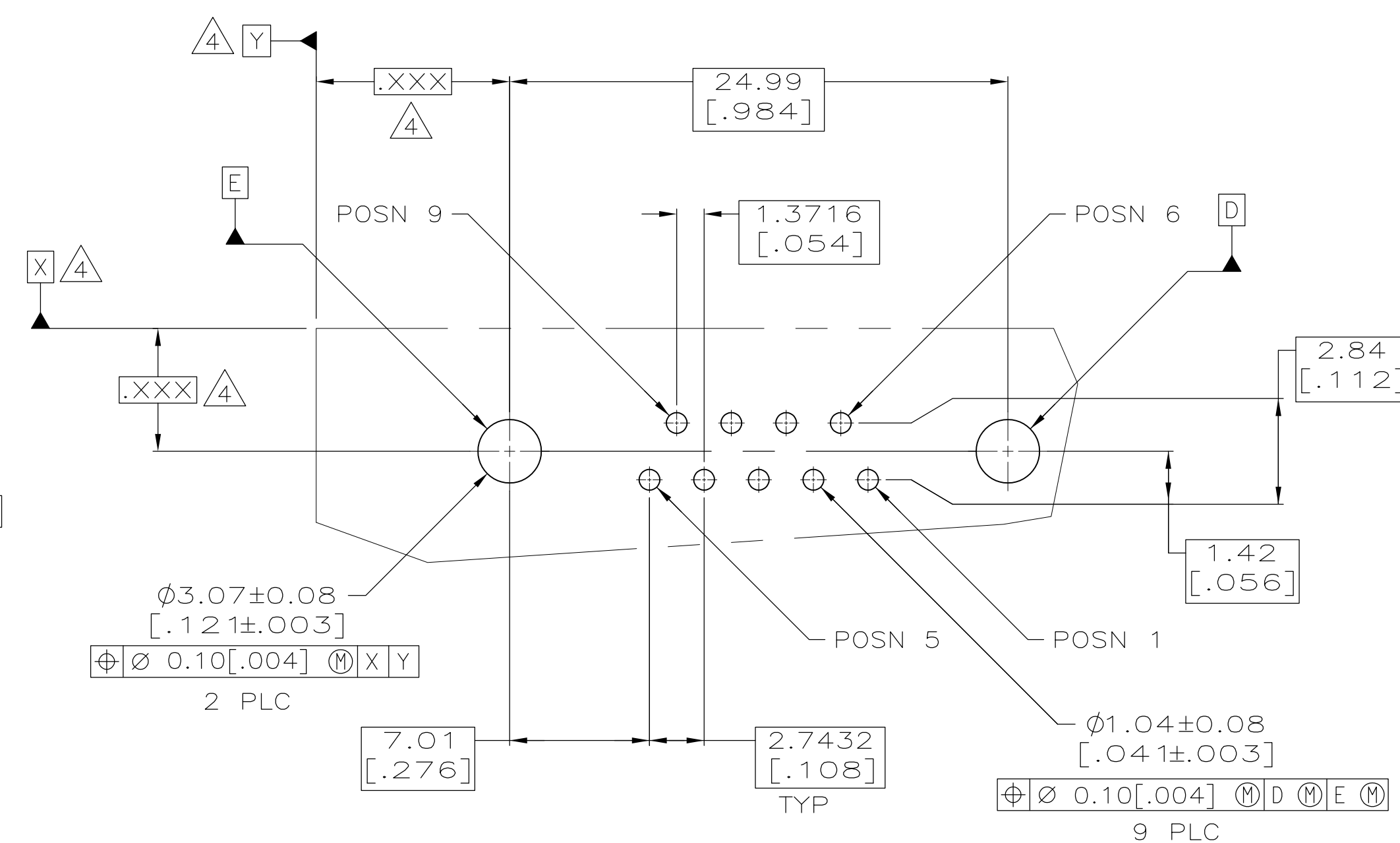
RECOMMENDED PC BOARD LAYOUT
