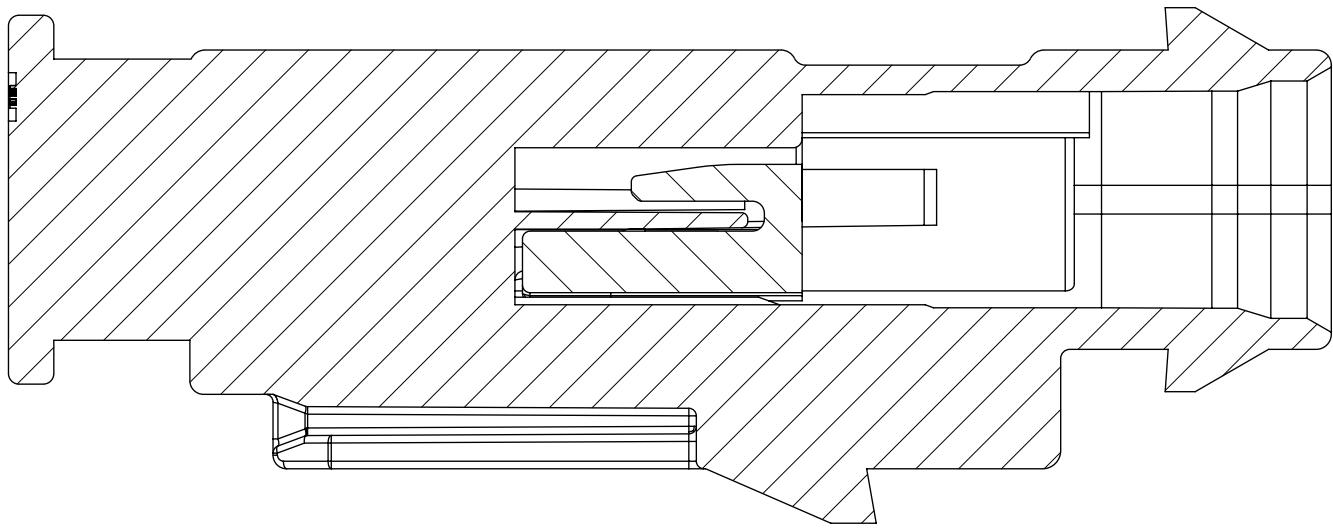
SECTION T-T
