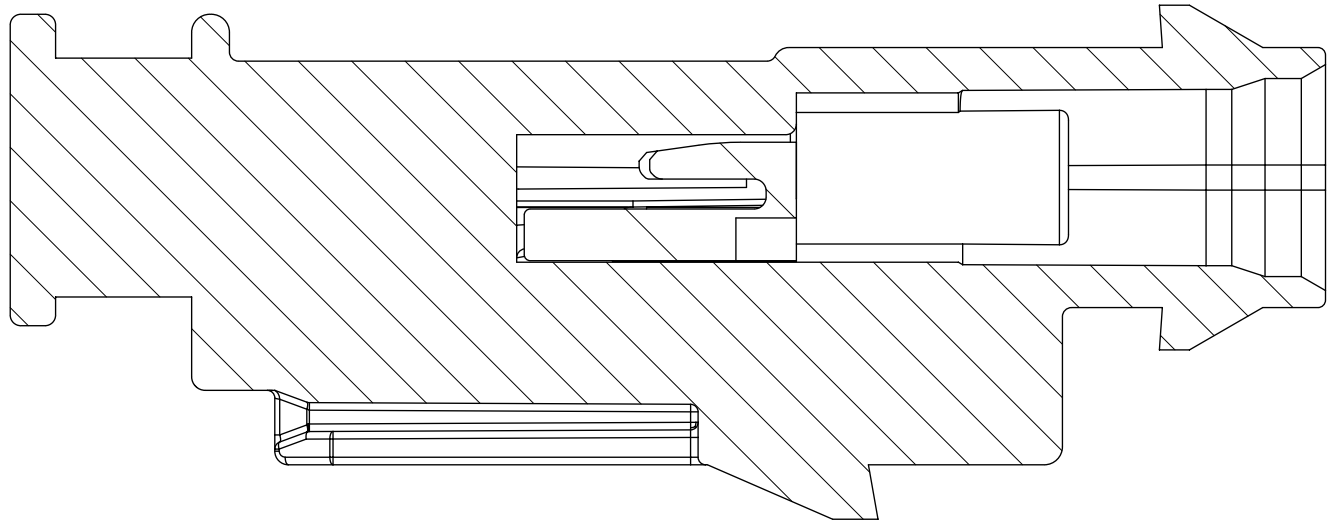
SECTION X-X
