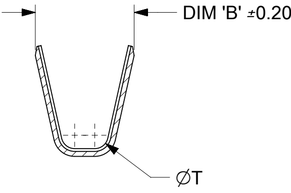
SECTION Y-Y
