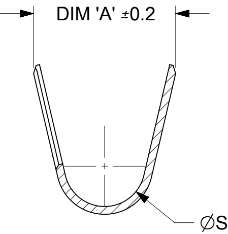
SECTION Z-Z
