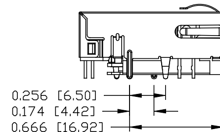
LEFT VIEW
