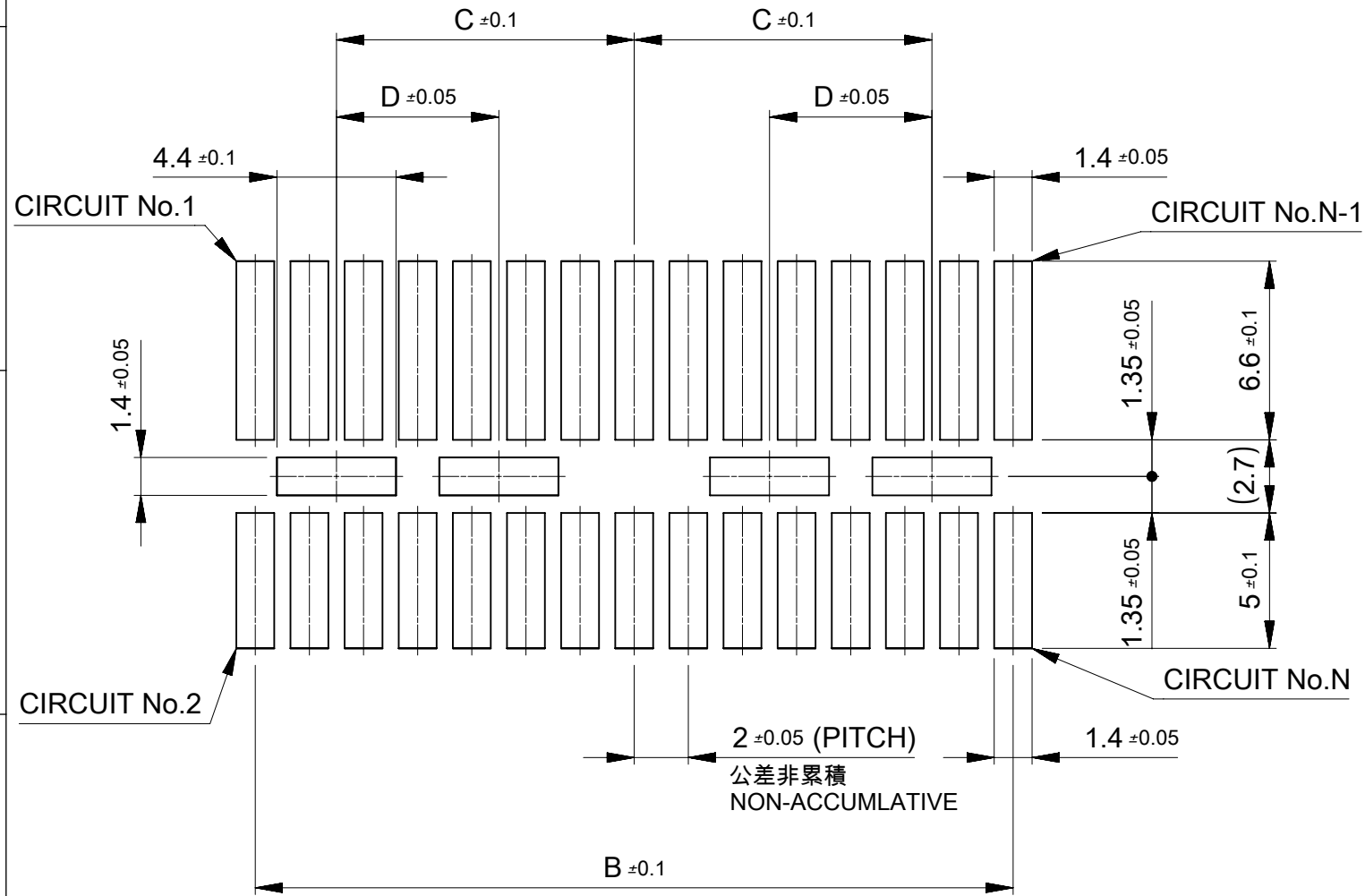
26P-30P (SCALE=4/1)
