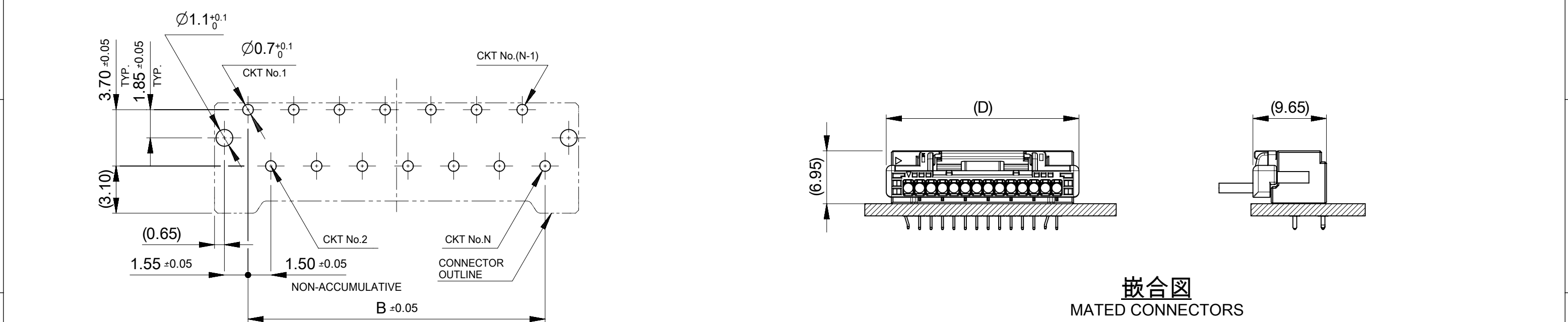
基板取付穴推奨寸法(マウント面) RECOMMENDED PCB HOLE DIMENSION (MOUNTING SIDE) (t=1.6)
