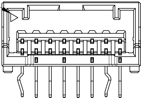
6~11極 6-11 CIRCUITS
