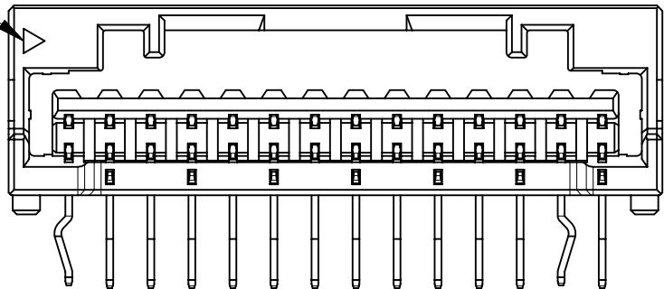
12~15極 12-15 CIRCUITS
