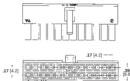
Receptacle Housing
