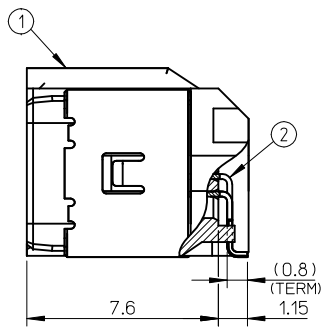
SECTION Z-Z
