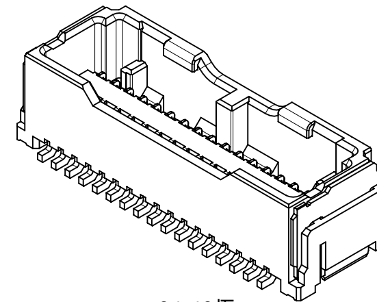
34-40極 34-40 CIRCUIT
