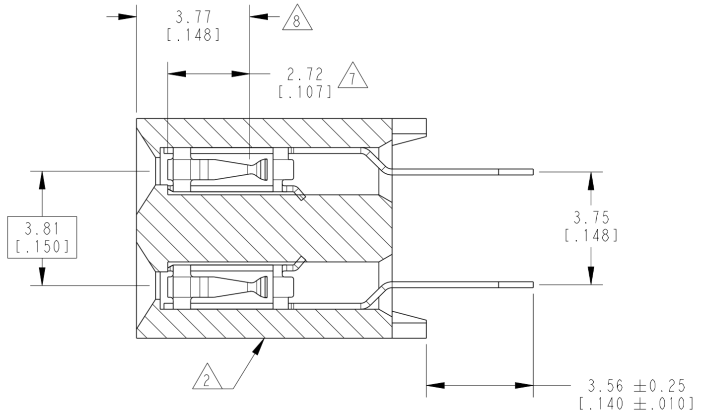
SECTION Z-Z SCALE 8:1
