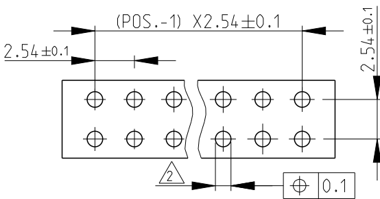
RECOMENDED PCB-LAYOUR FOR ACTION PIN ZONE
