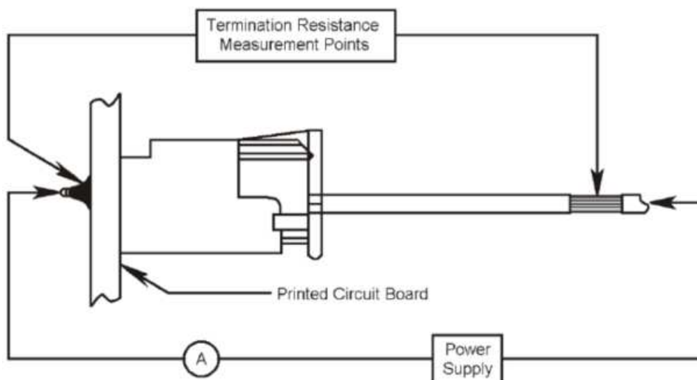
Figure 4 – Low Level Contact Resistance Measurement Points
