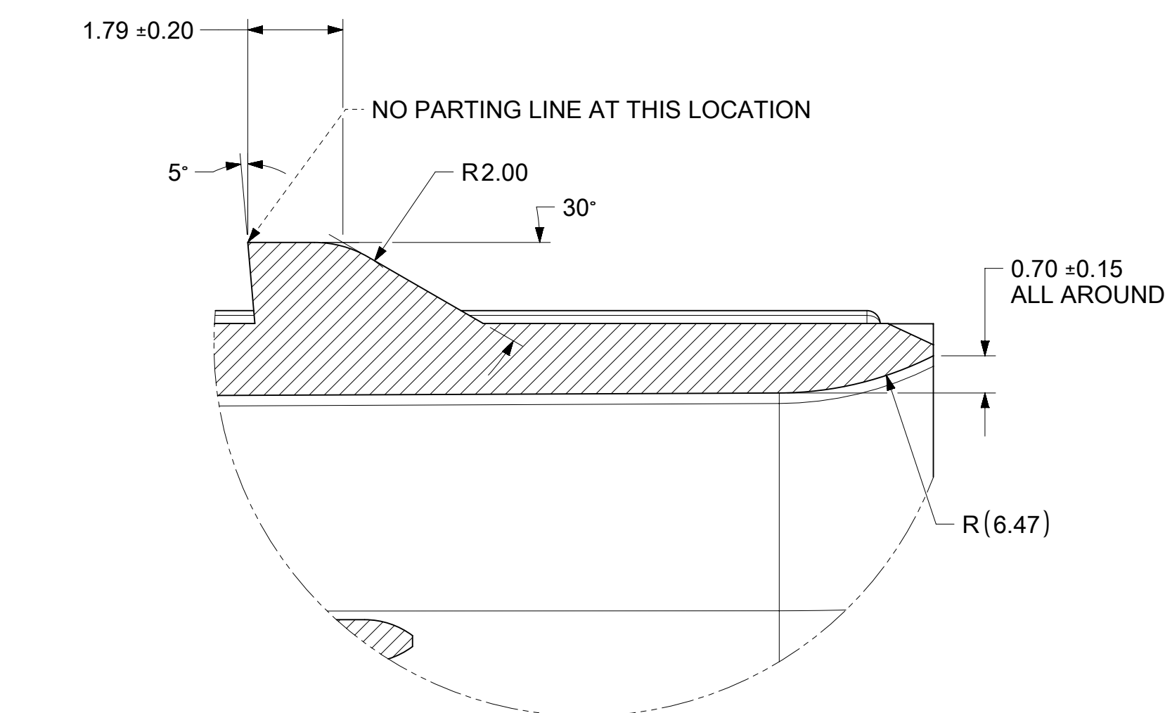
DETAIL 3 SCALE 10:1
