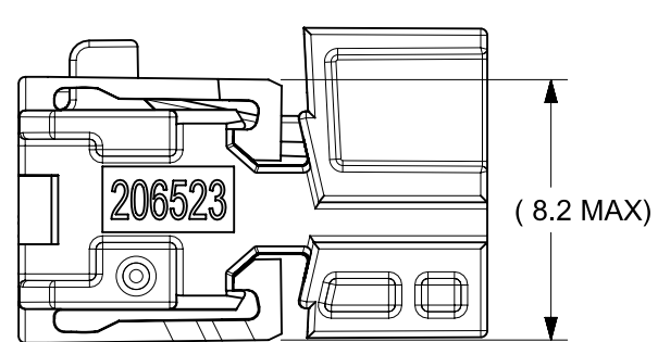
HINGE CLOSED
