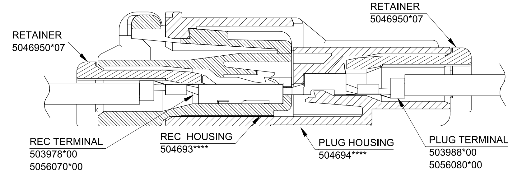
嵌合図 MATING CONNECTORES
