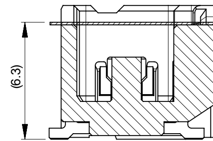
34-42極 34-42 CIRCUIT
