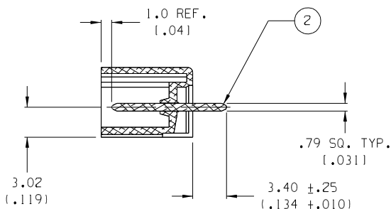
SECTION Z-Z
