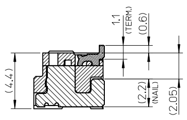
SECTION Z-Z
