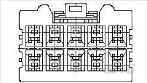
TE Part #1939984-1 GIC 3.3 PLUG HSG 10POS. 2ROW
