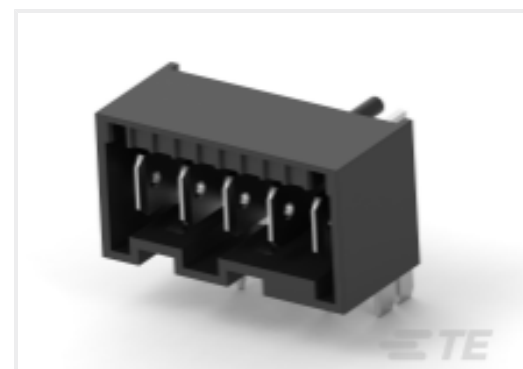
TE Part # 3-521384-5 ASSY PL R/A RAST5 HEADER 5P
