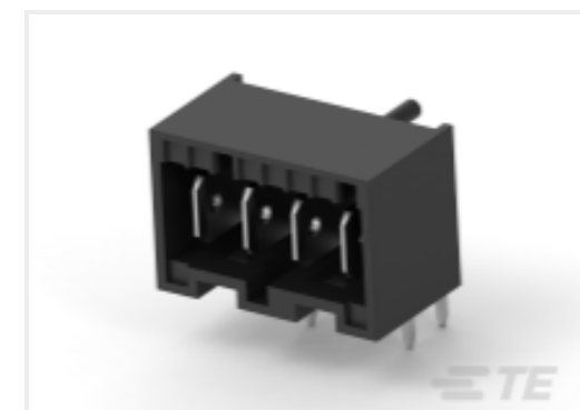
TE Part # 4-521384-4 ASSY PL R/A RAST5 HEADER 04-G
