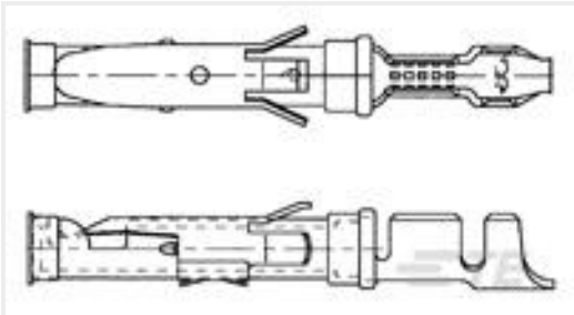
TE Part #163092-2 .062 DIA SOCKET ASSY 3+ (LP)
