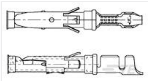
TE Part #163084-1 RECEPTACLE
