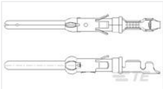
TE Part #163081-7 .062 DIA PIN ASSY 3+
