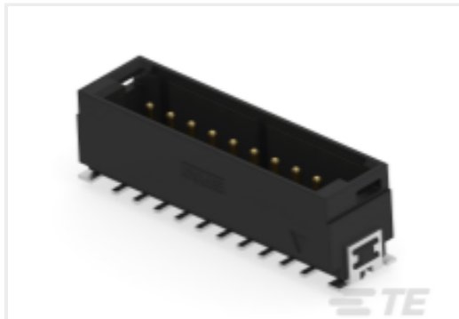
TE Part #464686-E DRCQ 2,54 20 M * SMD * 137 E012 094 GU-H
