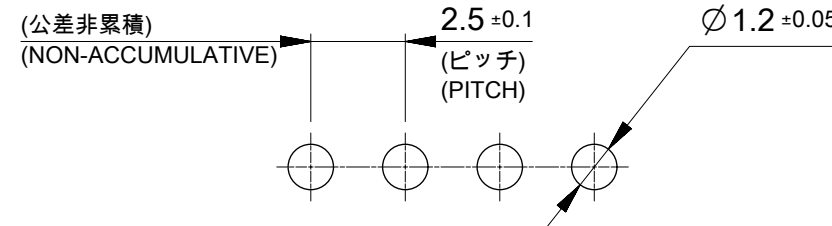
基板取付穴推奨寸法 RECOMMENDED P.C. BOARD HOLE DIM.
