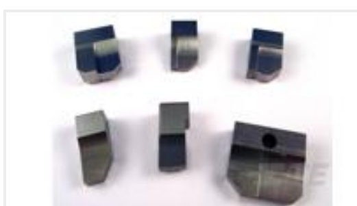
TE Part #1333217-1 ANVIL, E/FEED (.090)
